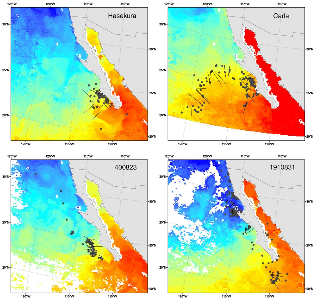
Fig. 2. Four examples of the virtual transects used to identify biologically relevant SST gradients transects across sea turtle and blue whale trajectories in 9 km weekly (8 day) AVHRR.
