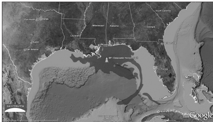
Figure 4. Graphic showing the cumulative oil-slick footprint for the BP/Deepwater Horizon oil spill, created by overlaying all of the oil slicks mapped by SkyTruth on satellite images taken between April 25 and July 16, 2010.
